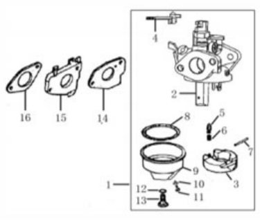
(CARBURETOR)
