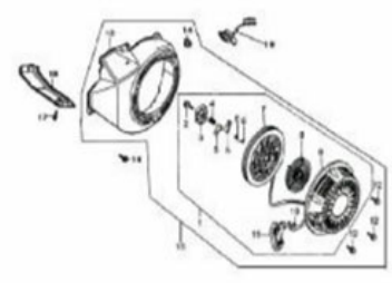
(Starter)
