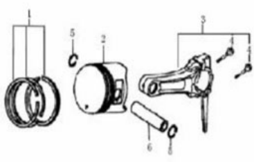
(Piston/connecting rod)
